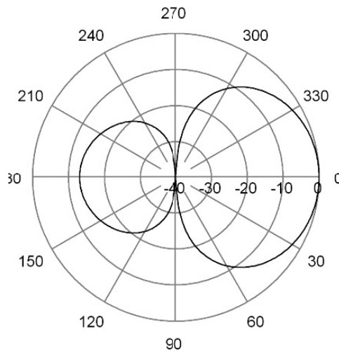
E-Plane | 73 MHz
