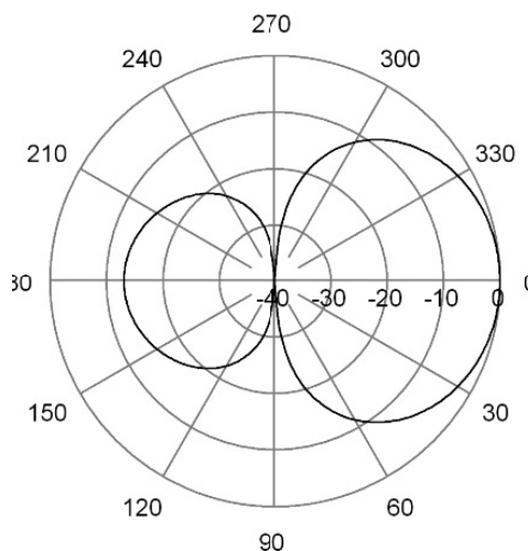
E-Plane | 102 MHz
