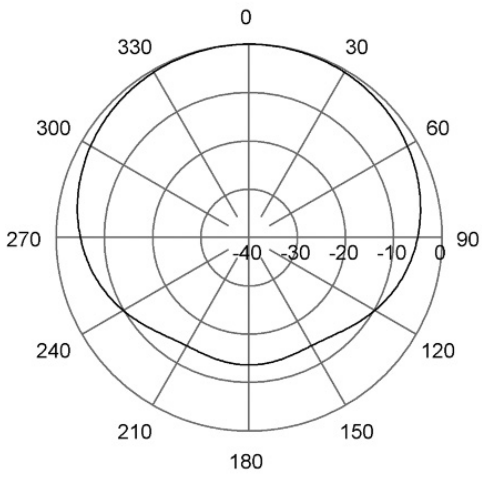
TYPICAL RADIATION PATTERN (H-PLANE - 82 MHZ)
