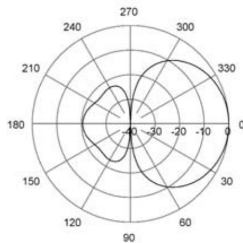
E-Plane | 144 MHz
