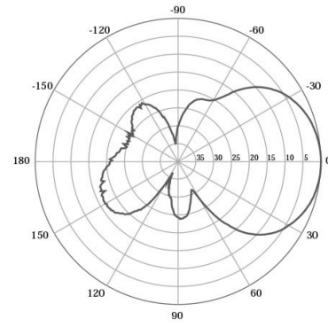
E-Plane | 405 MHz
