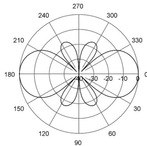
E-Plane | 156 MHz
