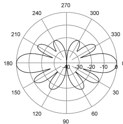
E-Plane | 435 MHz
