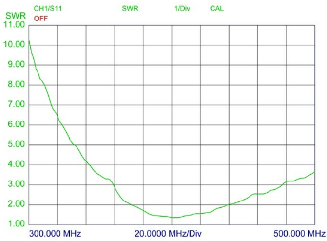
TYPICAL VSWR CURVE MP-B/450/445
