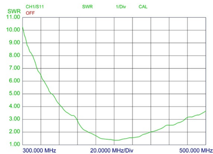
TYPICAL VSWR CURVE MP-B/450/445
