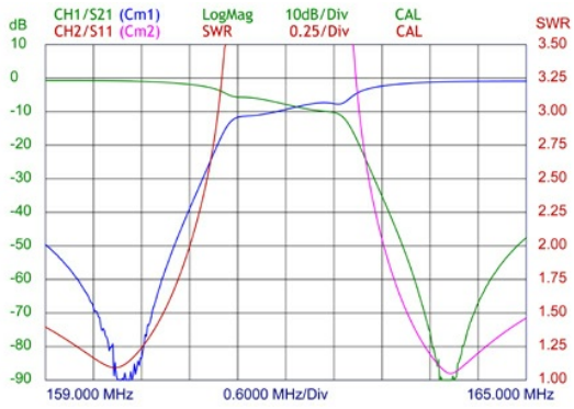
TYPICAL RESPONSE CURVE @ 5 MHz DUPLEX SPACING
